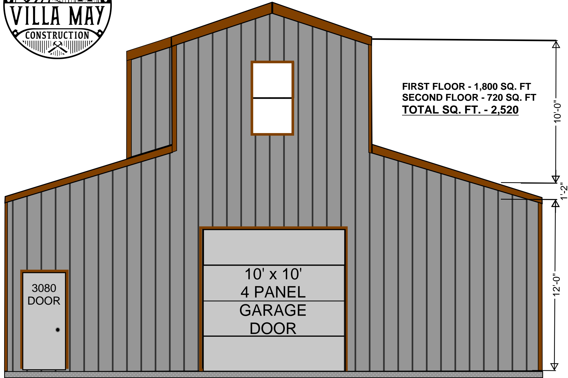
FRONT ELEVATION
